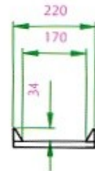
RIGHT HAND RAMP (shown open and folded for stowage)
